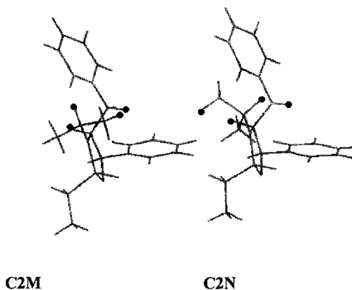
Fig. 3. Minimised (C2M) and NOE (C2N) conformers of compound 9; the dots refer to the hydrogen atoms giving raise to NOE.
