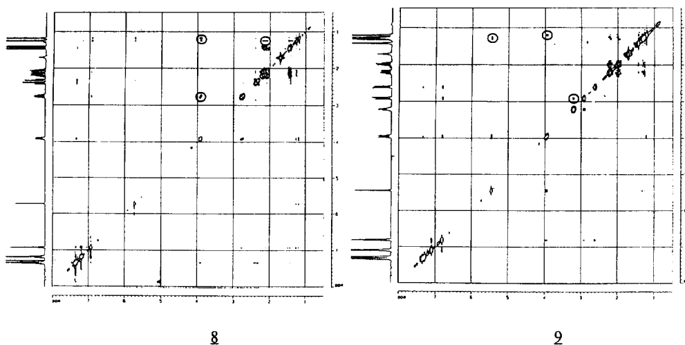
Fig. 4. NOESY spectra of compounds 8-9 ; circled atoms corresponds to NOE signals
